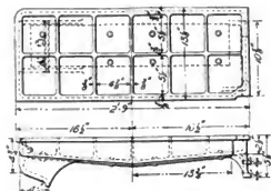
Figs. 561-563. Deal Plate for Grate.
